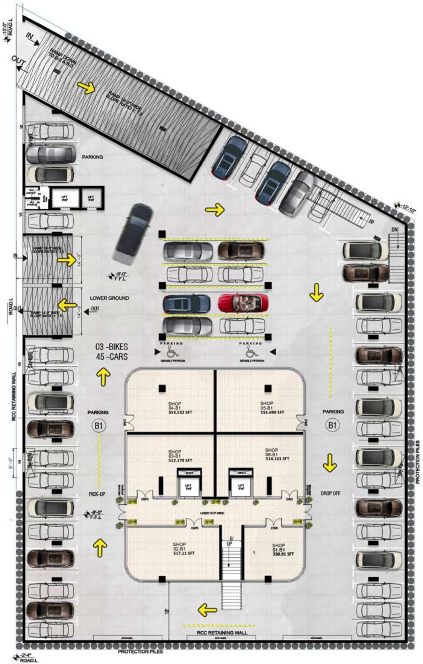
FIRST BASEMENT FLOOR PLAN
