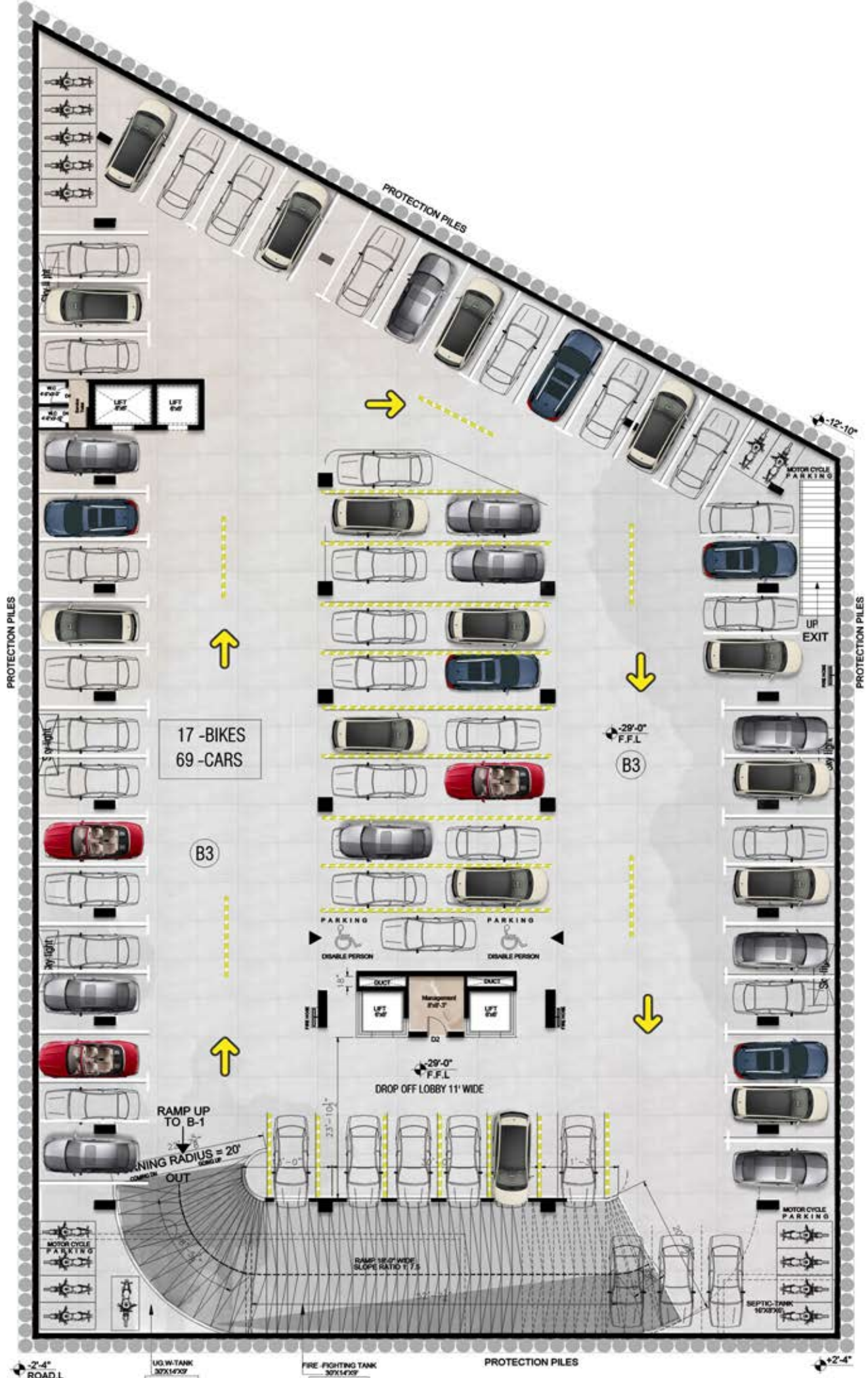
THIRD BASEMENT FLOOR PLAN
